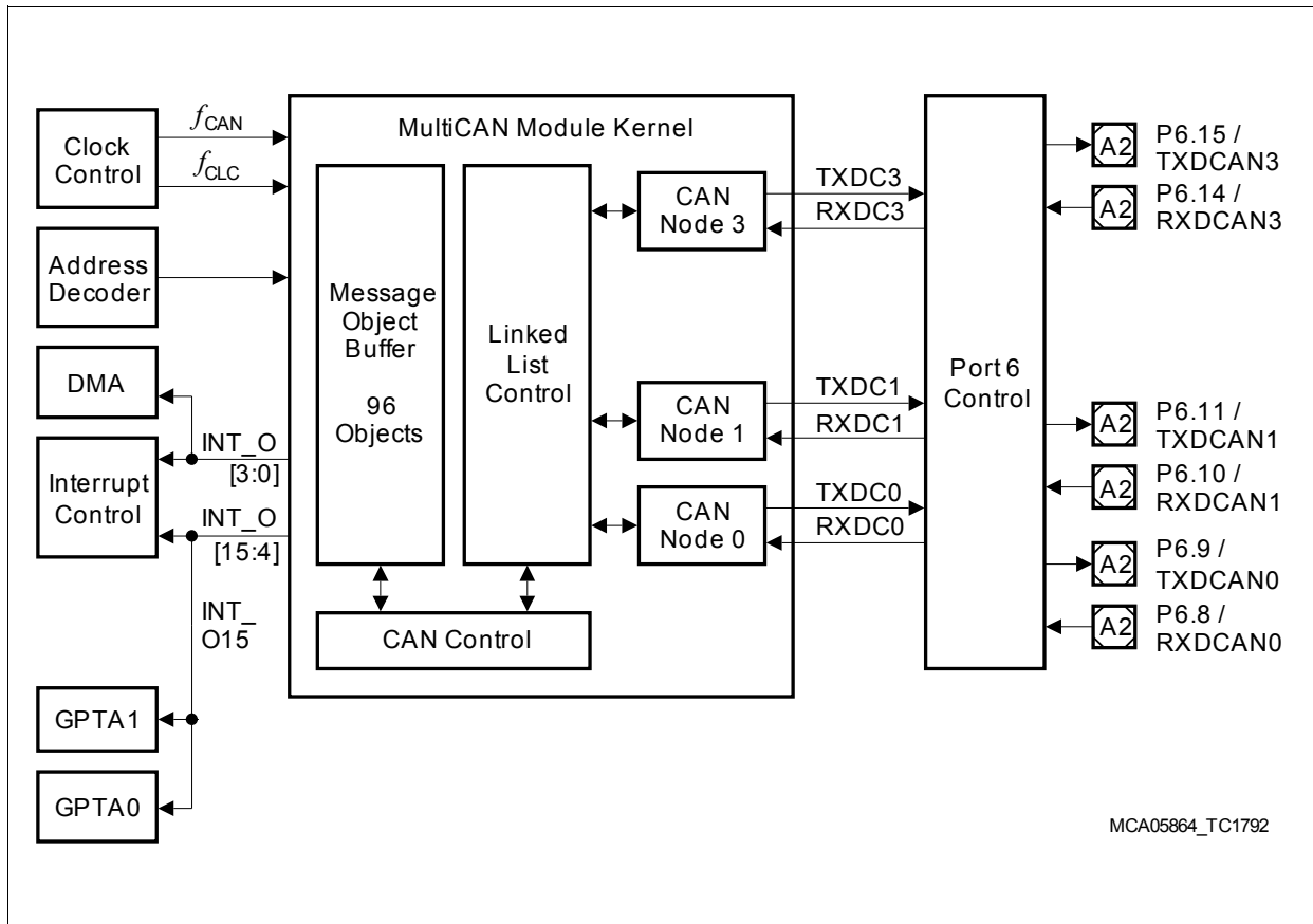
Figure 11 Block Diagram of MultiCAN Module with Time-Triggered Extension
