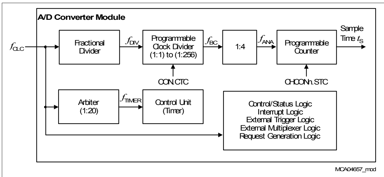
Figure 22 ADC0/ADC1 Clock Circuit
