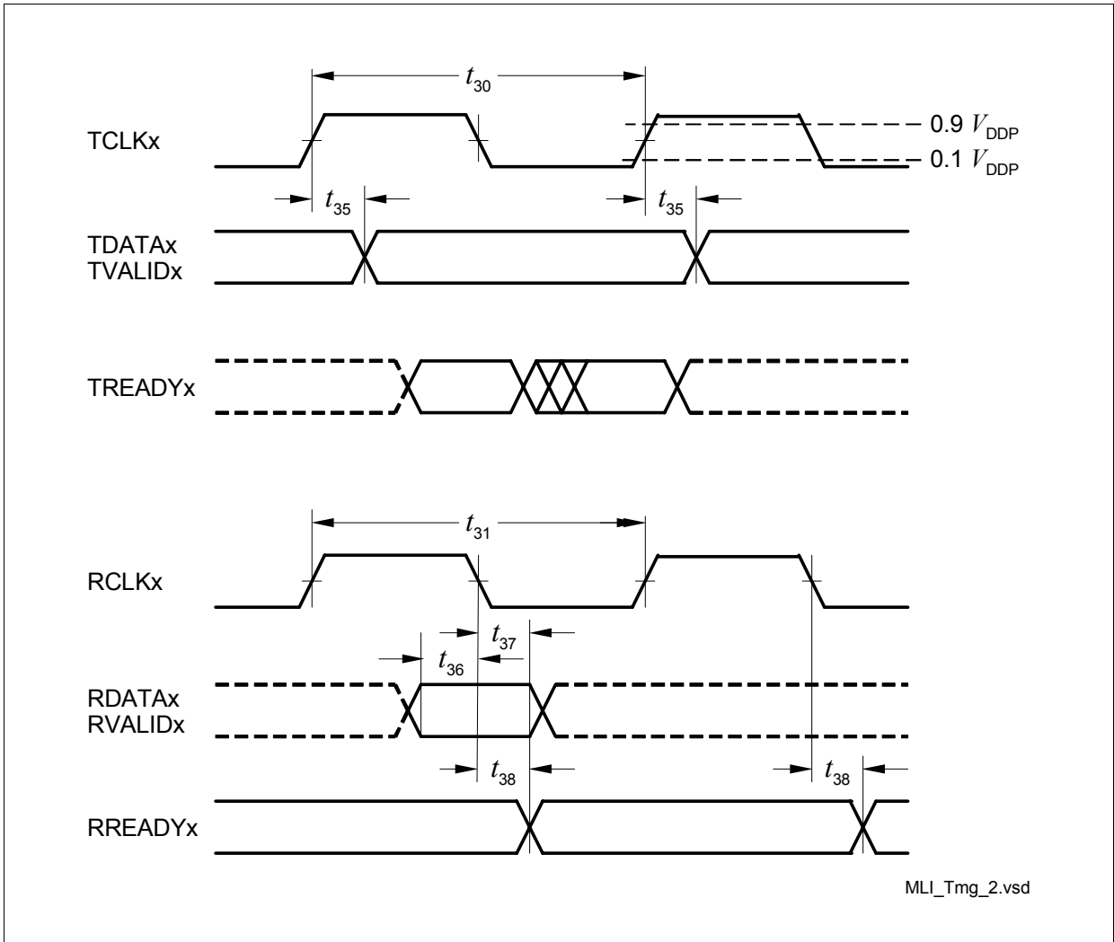
Figure 40 MLI Interface Timing
