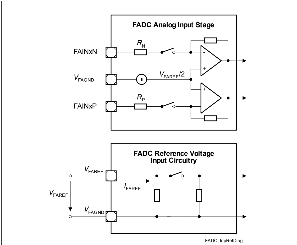
Figure 25 FADC Input Circuits
