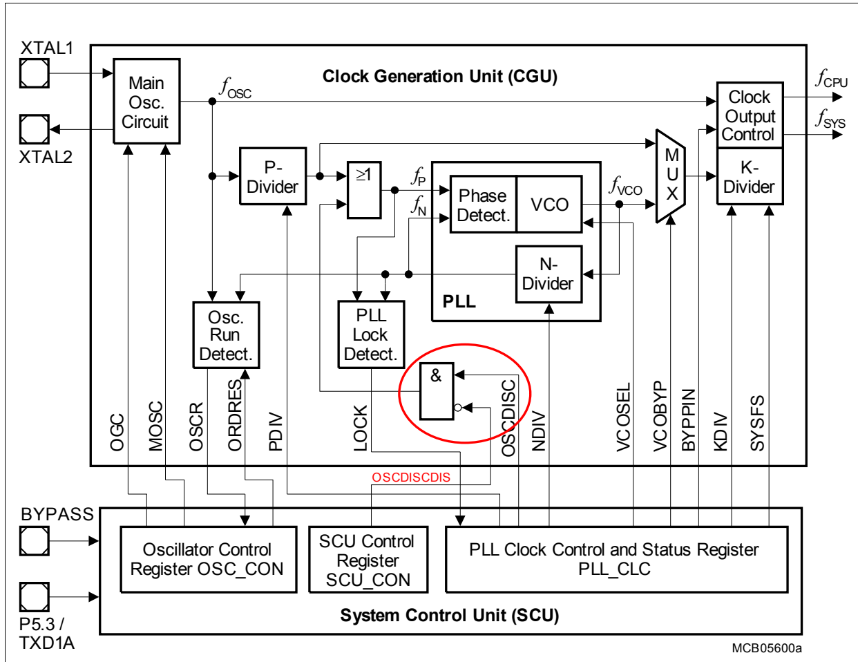
Figure 19 Clock Generation Unit (the red signal available only in the -AB step)
