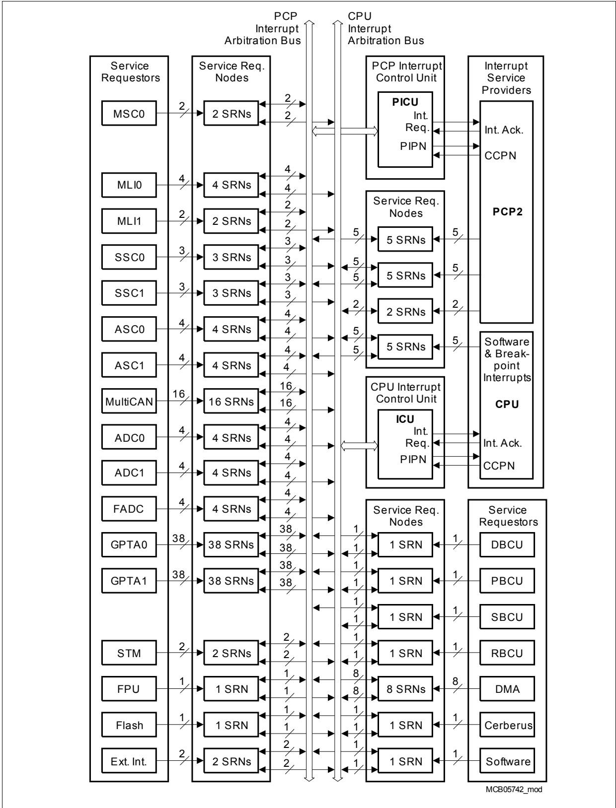
Figure 7 Block Diagram of the TC1792 Interrupt System
