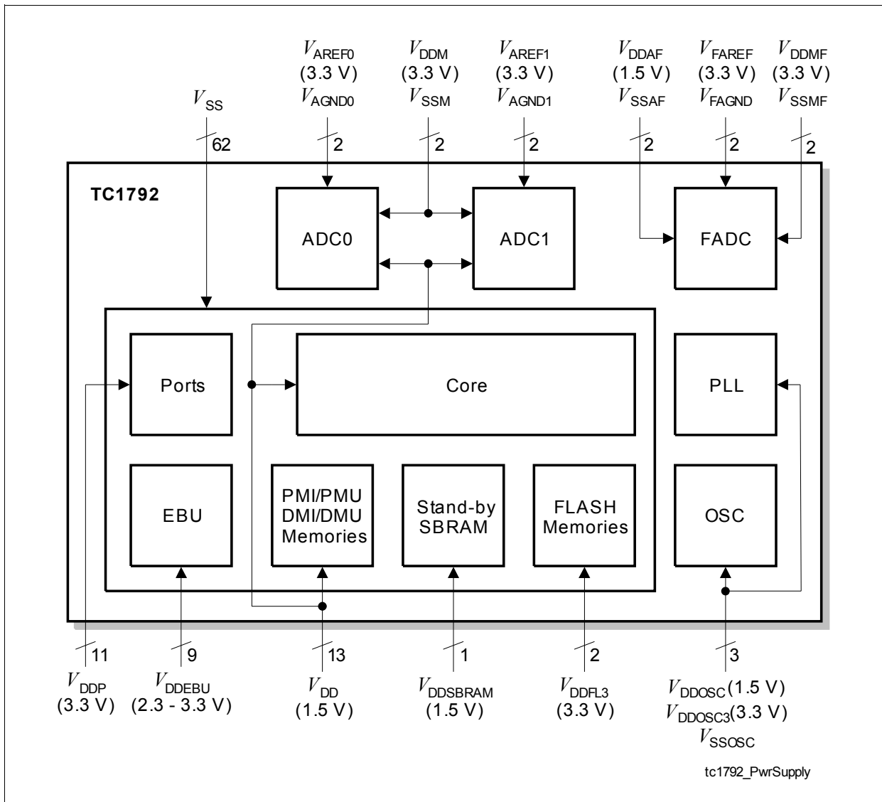
Figure 21 Power Supply Concept of TC1792
