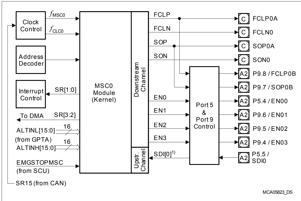
Figure 10 Block Diagram of the MSC Interface
