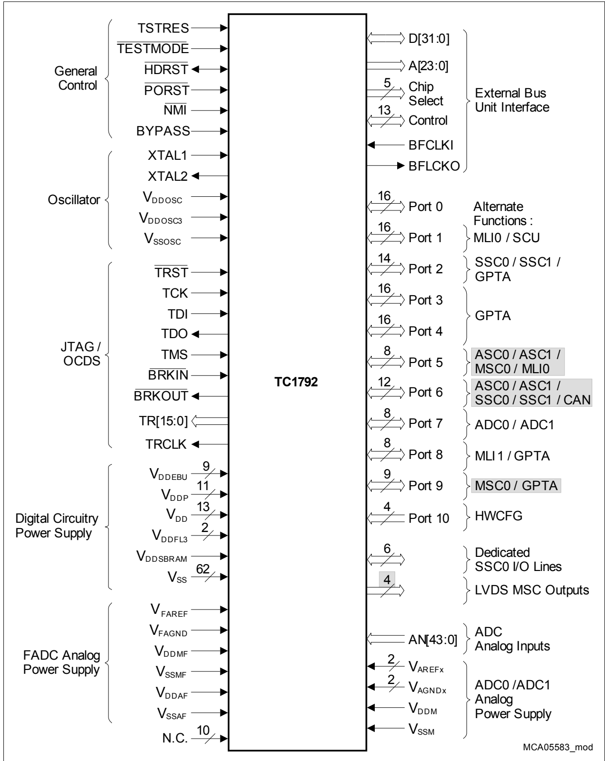
Figure 2 TC1792 Logic Symbol
