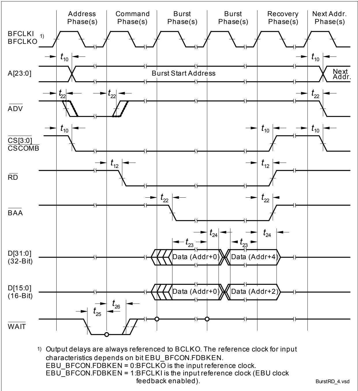
Figure 38 EBU Burst Mode Read Timing
