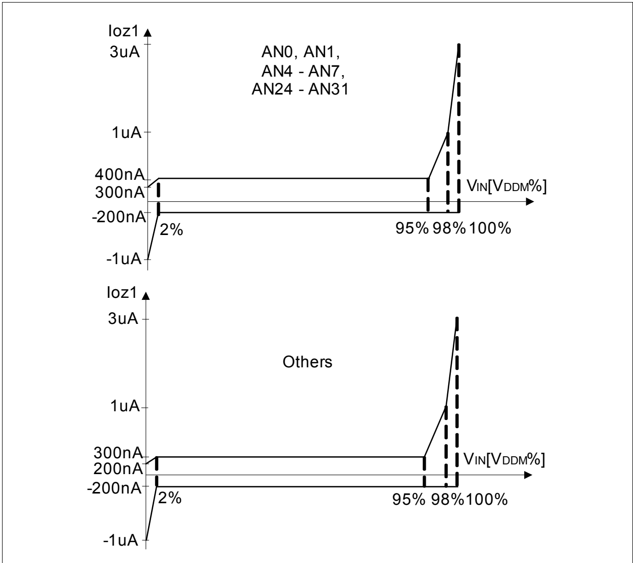
Figure 24 ADC0/ADC1 Analog Inputs Leakage
