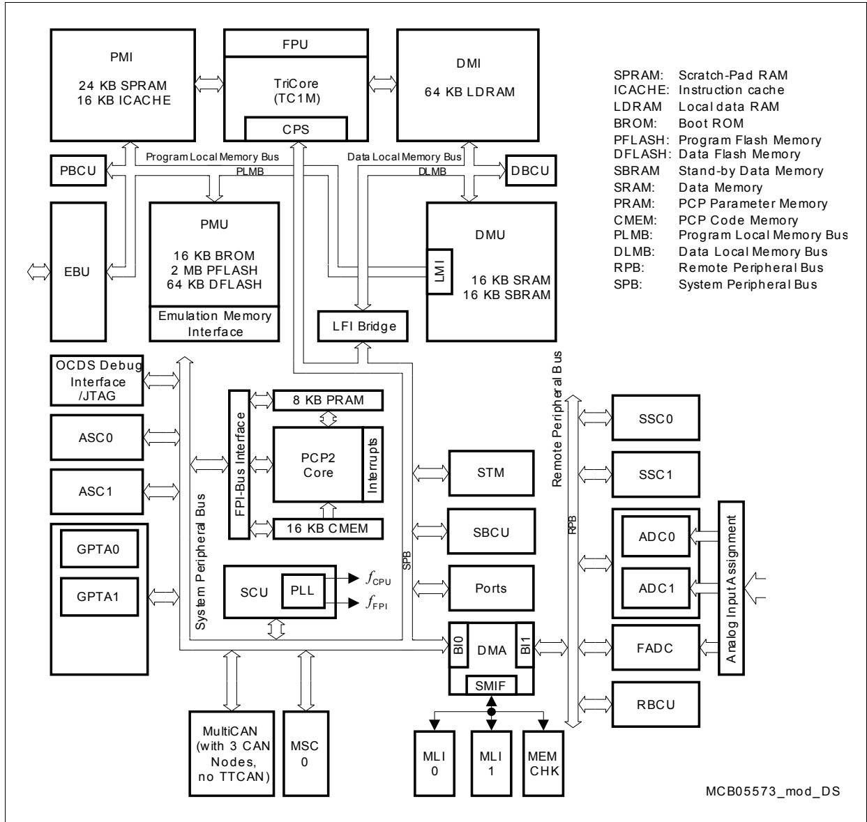
Figure 1 TC1792 Block Diagram
