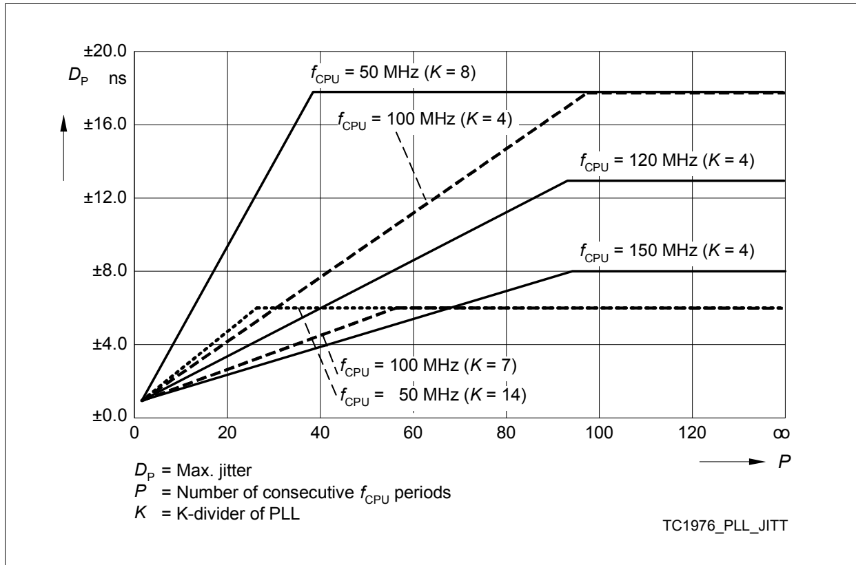
Figure 32 Approximated Maximum Accumulated PLL Jitter for Typical CPU Clock Frequencies f_{\text{CPU}} (overview)
