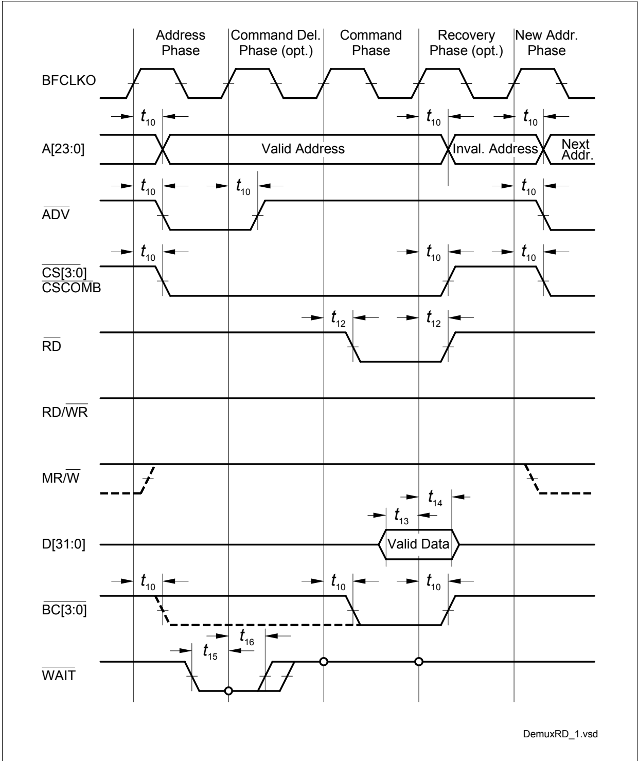
Figure 36 EBU Demultiplexed Read Timing
