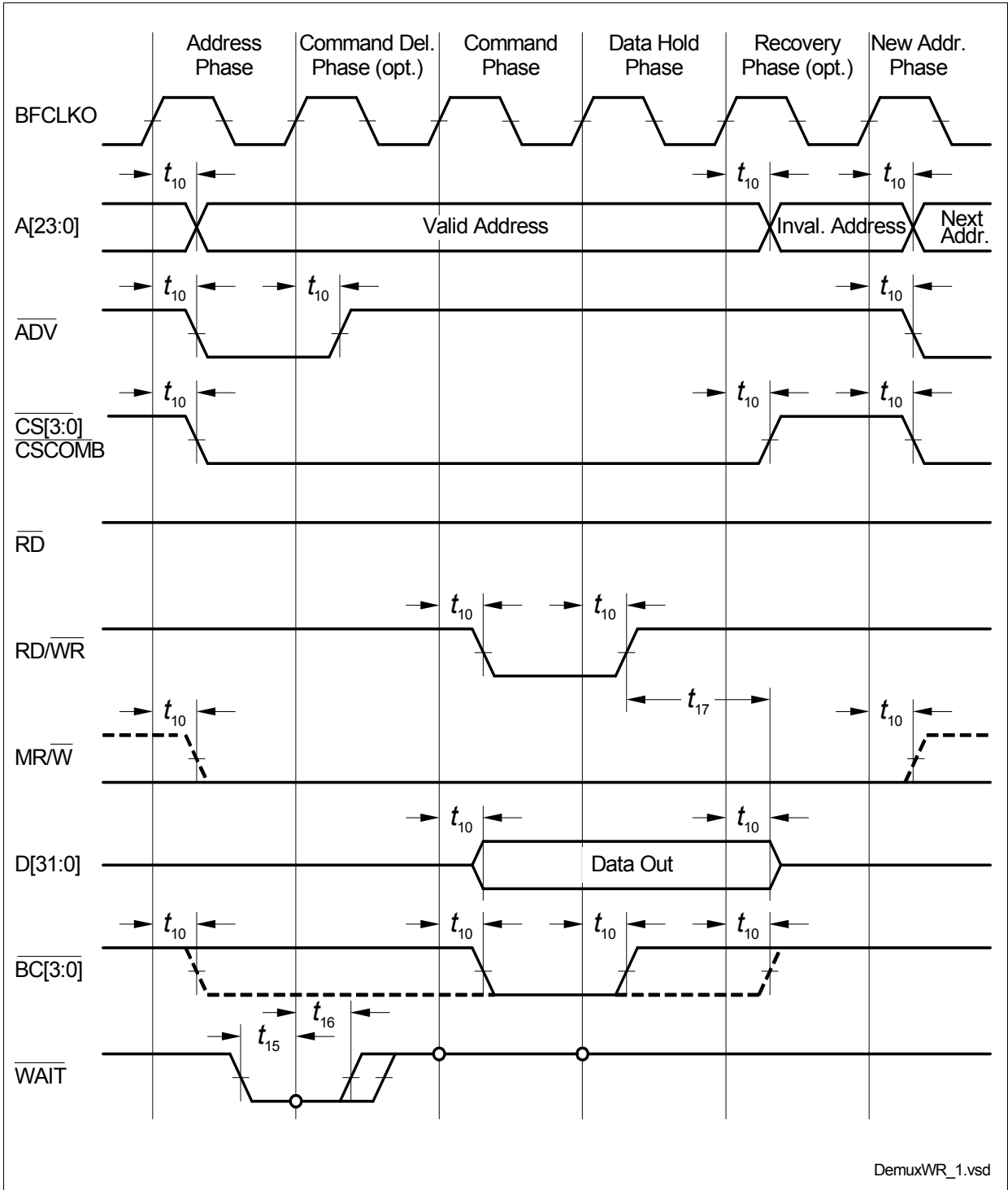
Figure 37 EBU Demultiplexed Write Timing
