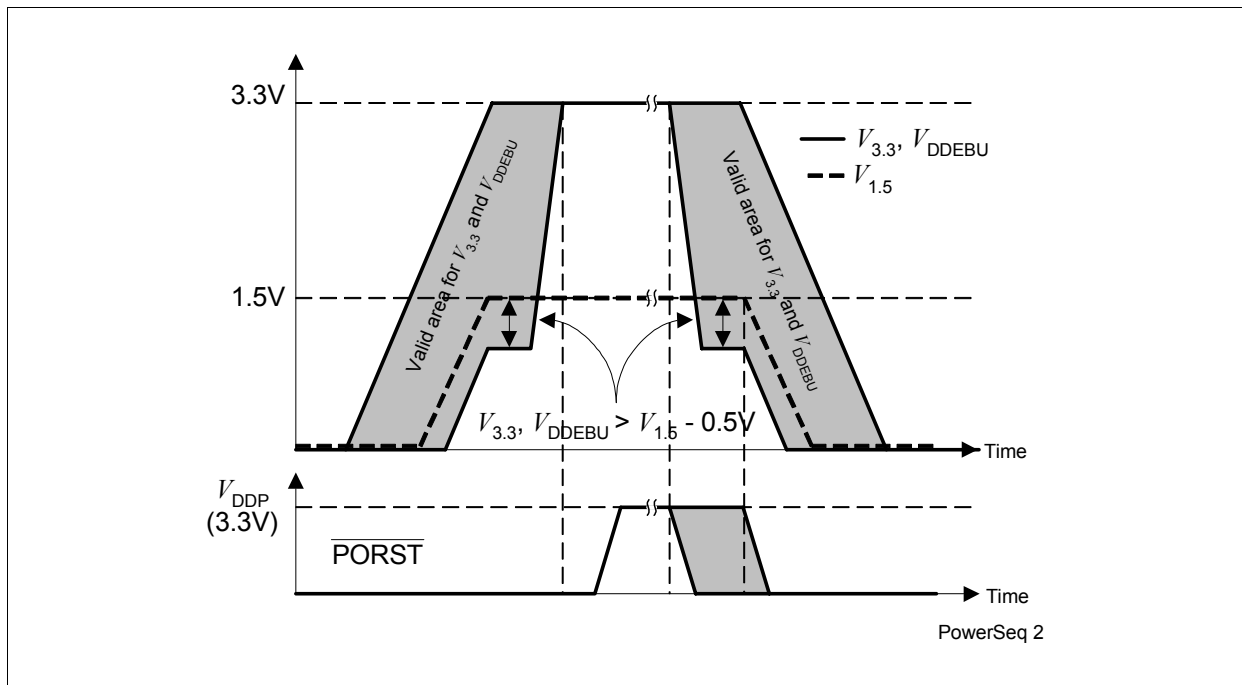
Figure 29 V_{DDP} / V_{DDEBU} / V_{DD} Power Up Sequence
