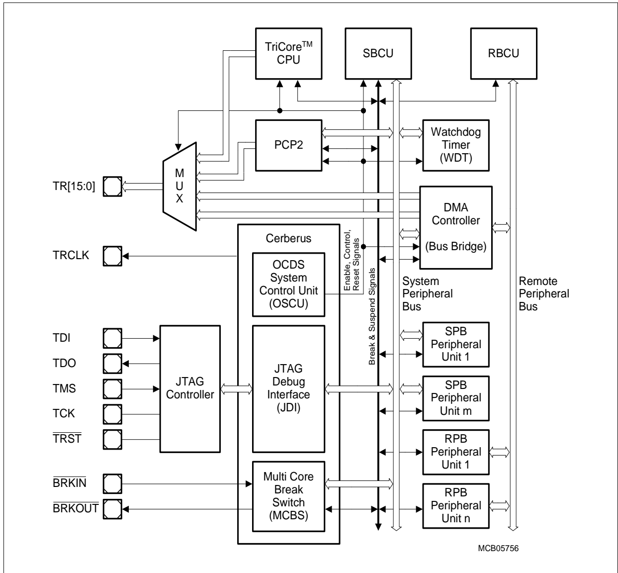
Figure 18 OCDS System Block Diagram
