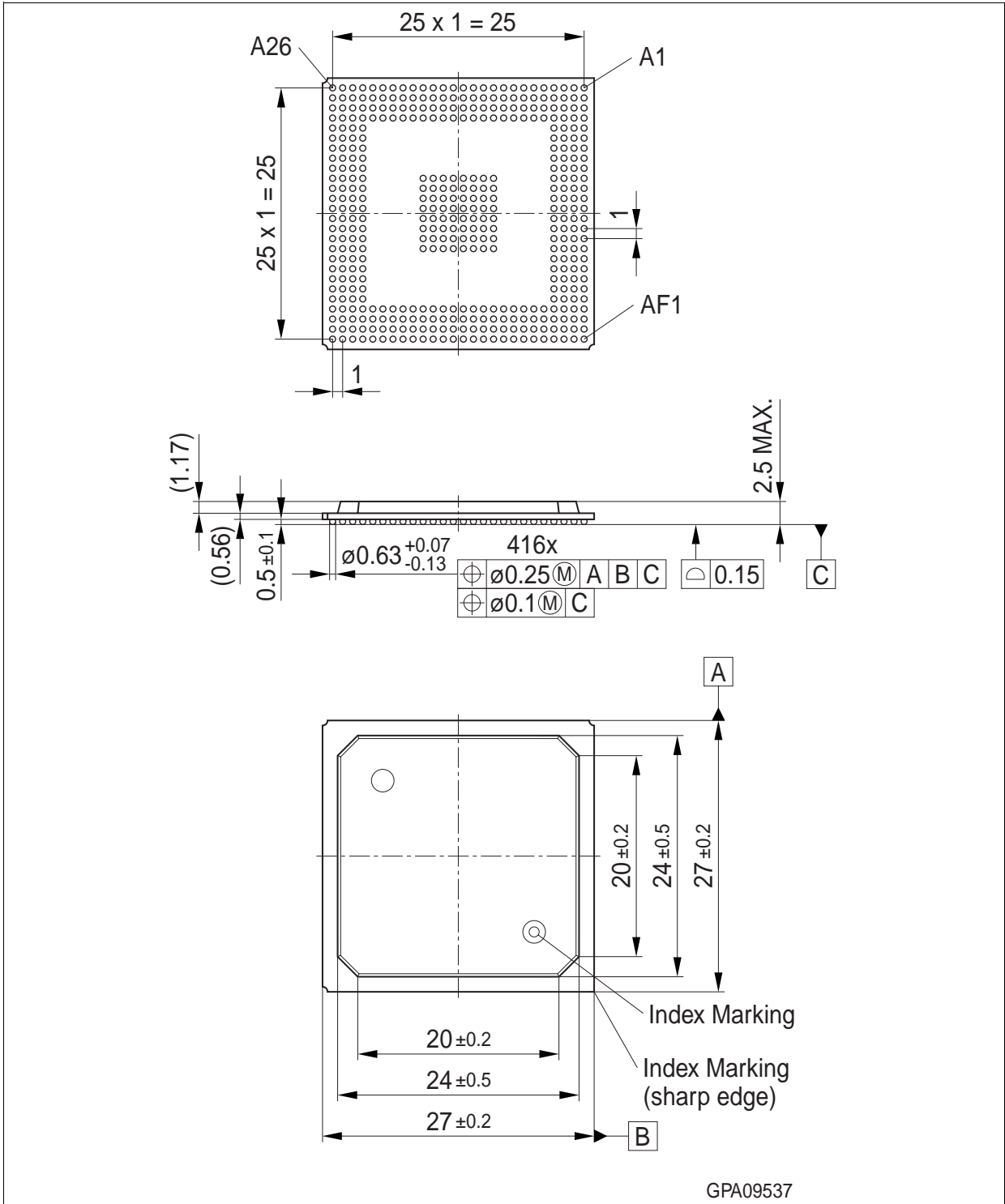
Figure 43 P-BGA-416-4, Plastic Low Profile Pitch Ball Grid Array
