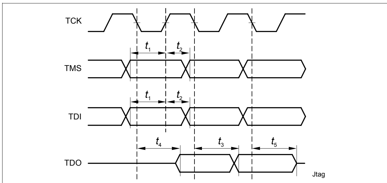
Figure 4-2 JTAG Timing
