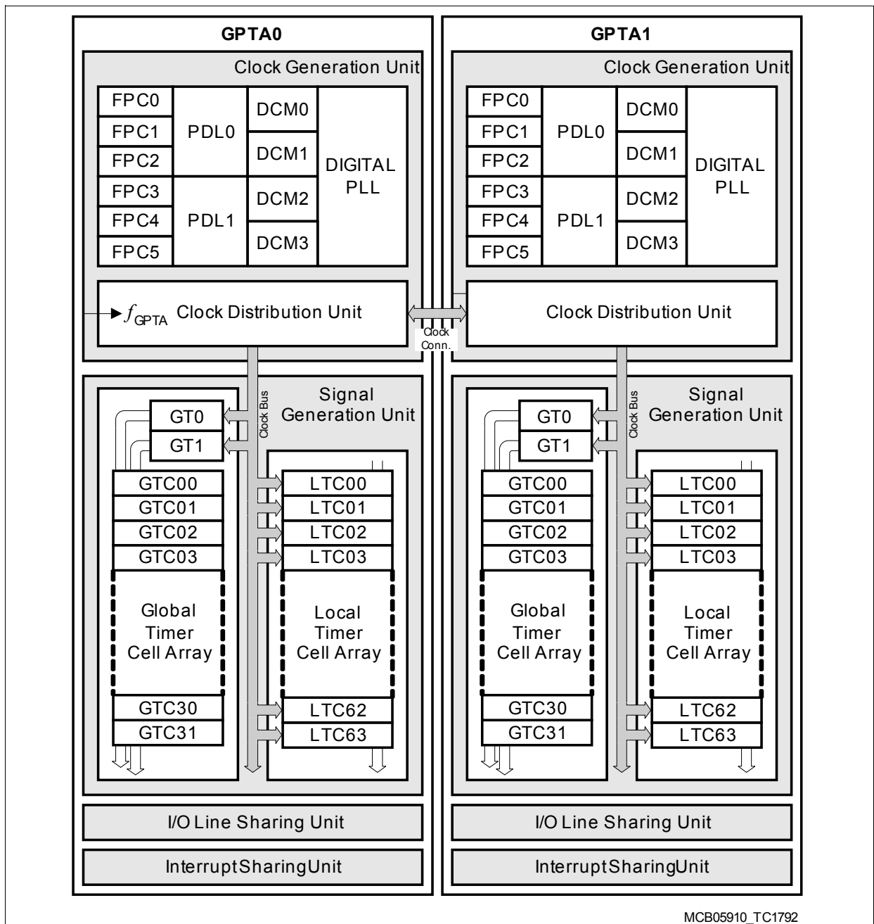
Figure 14 Block Diagram of the GPTA Modules
