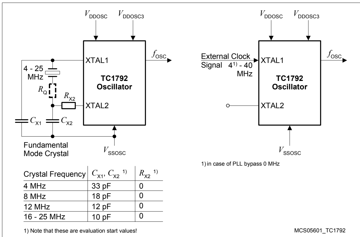
Figure 20 Oscillator Circuitries
