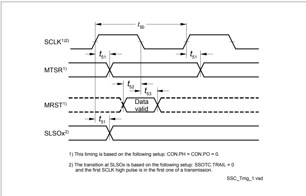
Figure 42 SSC Master Mode Timing
