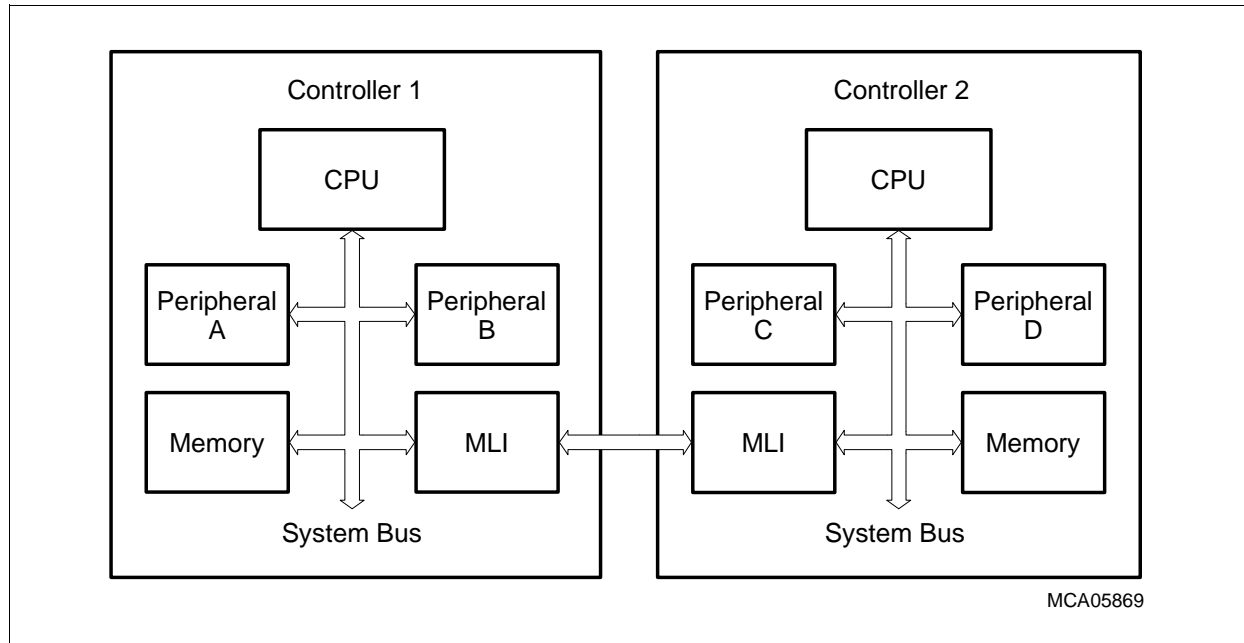
Figure 12 Typical Micro Link Interface Connection
