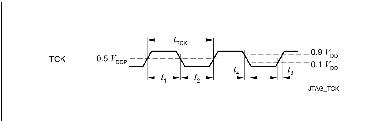
Figure 4-1 TCK Clock Timing
