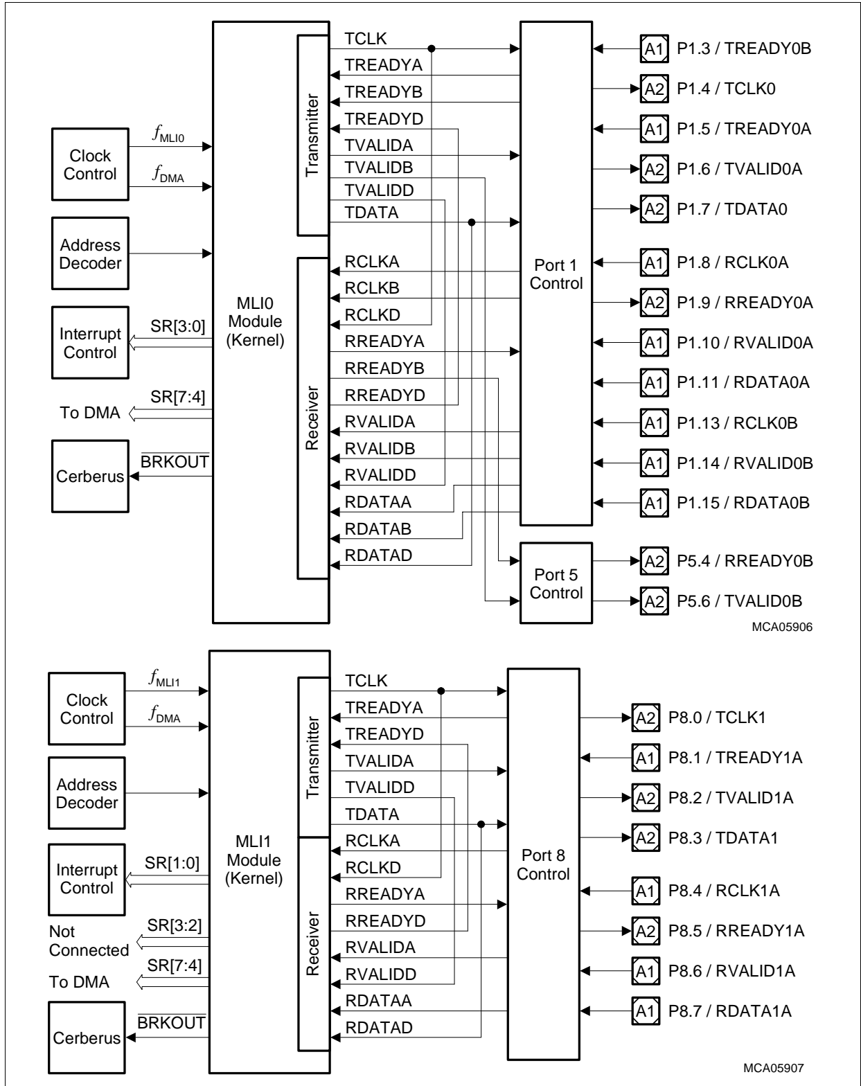
Figure 13 Block Diagram of the MLI Modules
